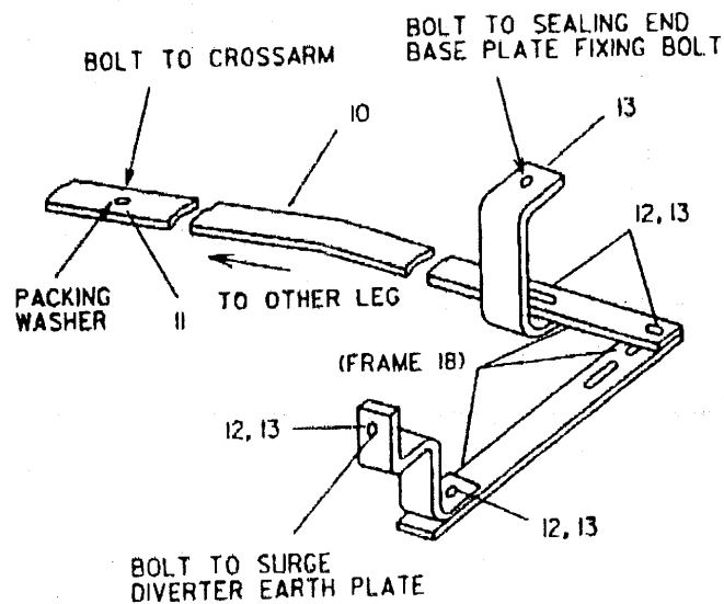
EARTH BAR ASSEMBLY
